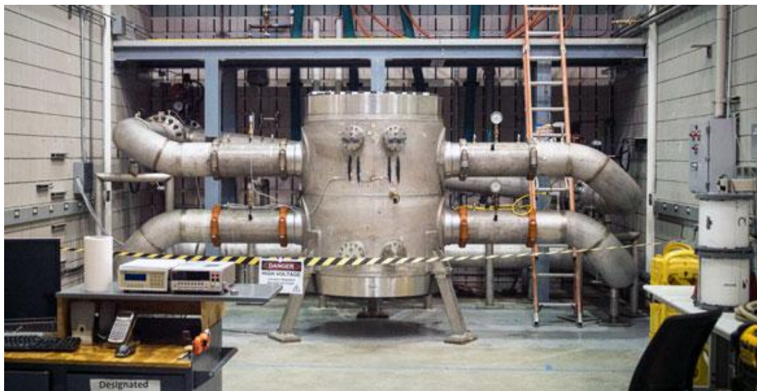
The new world-record magnet connected to cooling water pipes. Some 4,275 gallons of cold water flush through it per minute to keep it cool.
